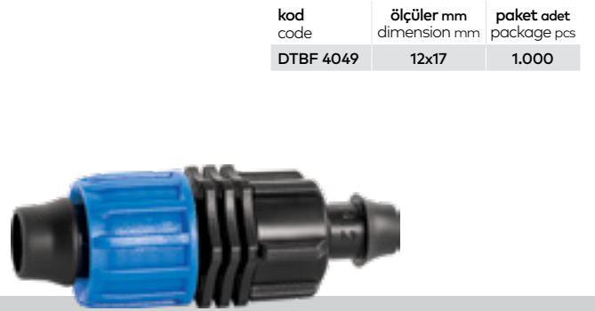
Contasız Vidalı Çıkış Nipelini Offtake Nipple with Nut (without Gasket)
